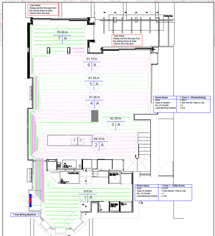
System RED pipe layout example
